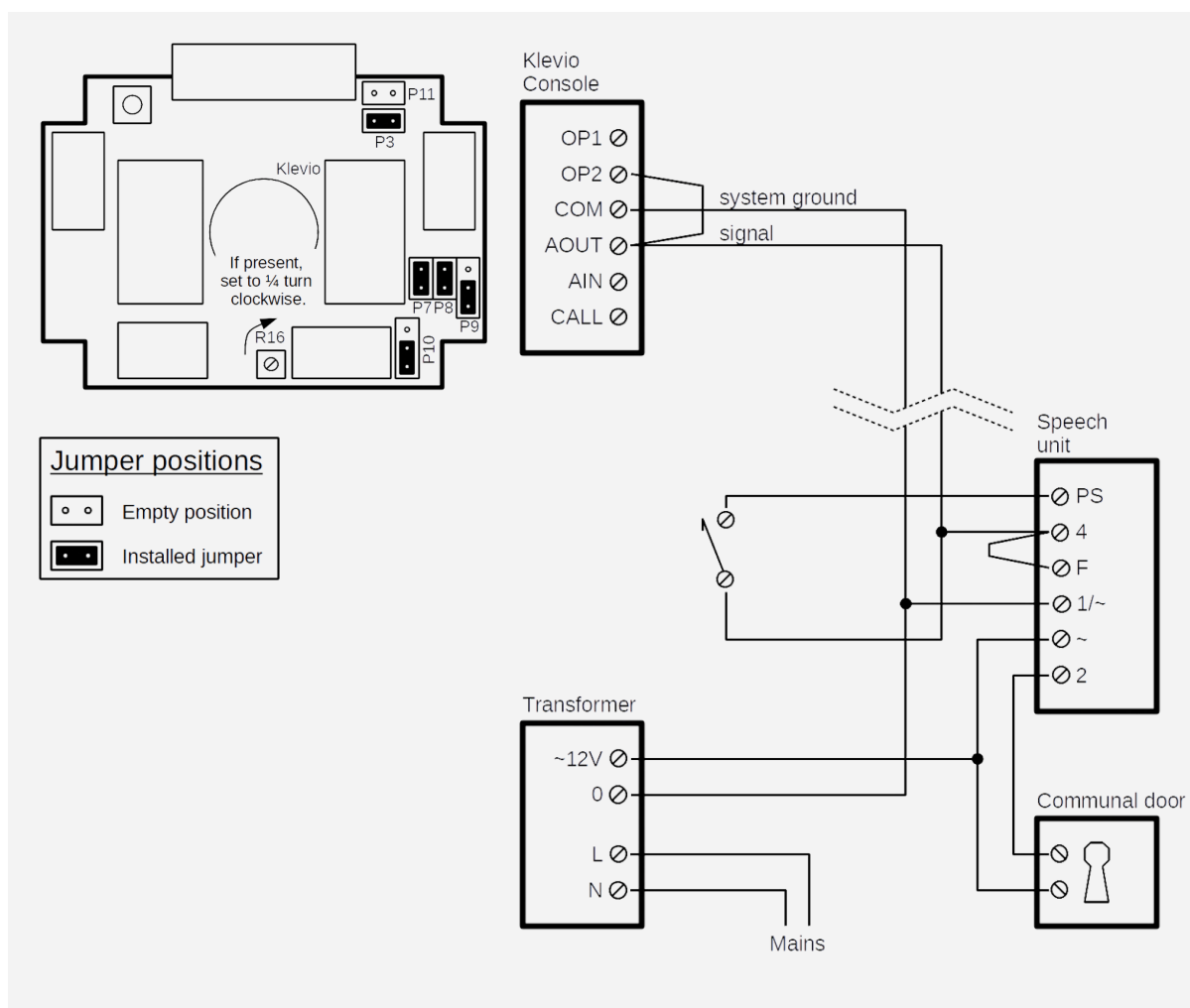
Fig. 12: Wiring Klevio Console v2.8 to a 2-wire analog system (1+n)
