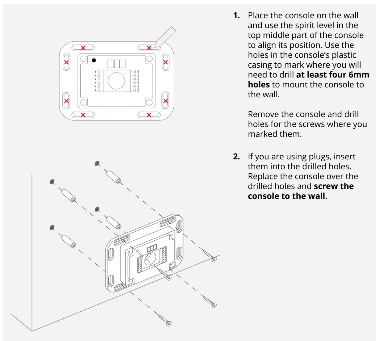
Fig. 9: Mounting the Klevio Console on a wall
