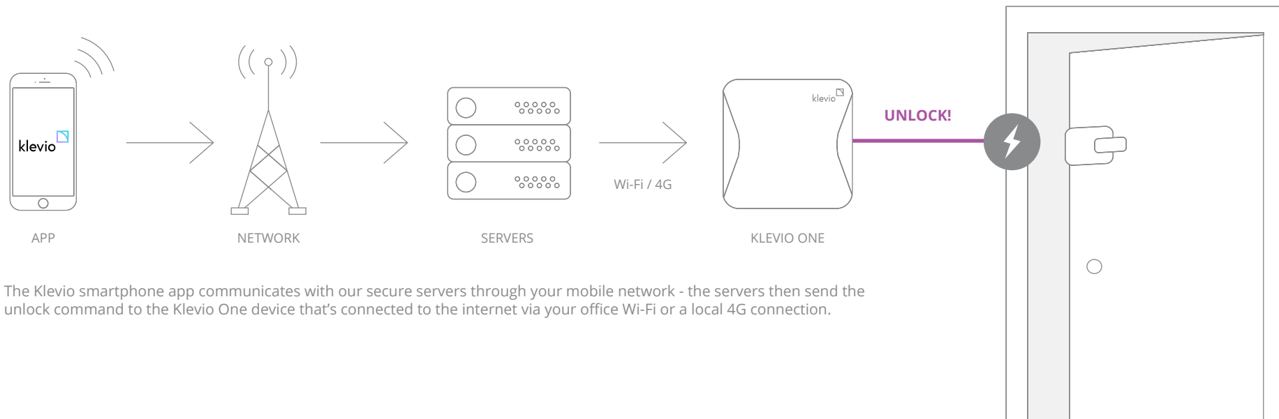
The Klevio device controls your lock via an electric strike and can connect to your existing access system as well
